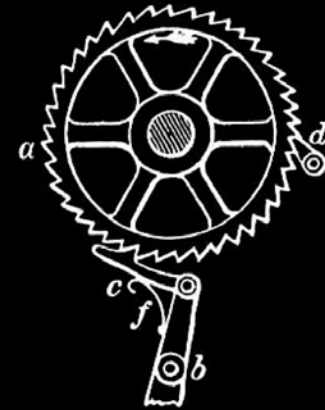
Ratchet-wheel. — a , the wheel; b , reciprocating lever; c , pawl conveying motion to wheel; f , spring; d , pawl preventing reversal of motion.
